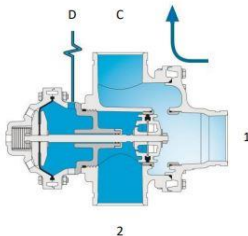
Outlet Valve Back-flush Mode
